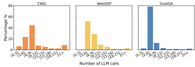
Figure 10: The proportion of question of PoG and PoG-E by different LLM Calls among CWQ, WebQSP, and GrailQA datasets
